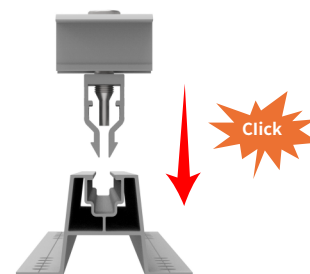
• WQ-IRE-3035 Universal End Clamp
