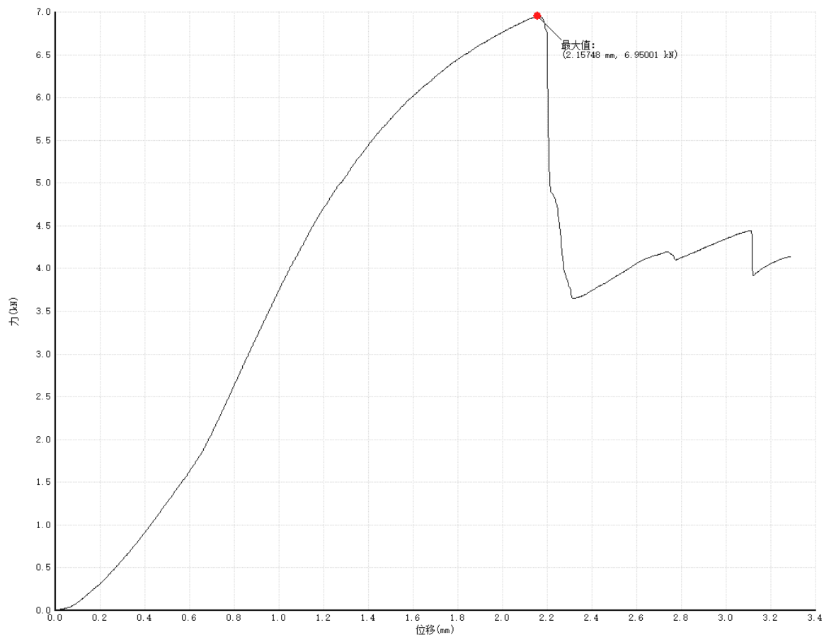
Force-displacement curve
