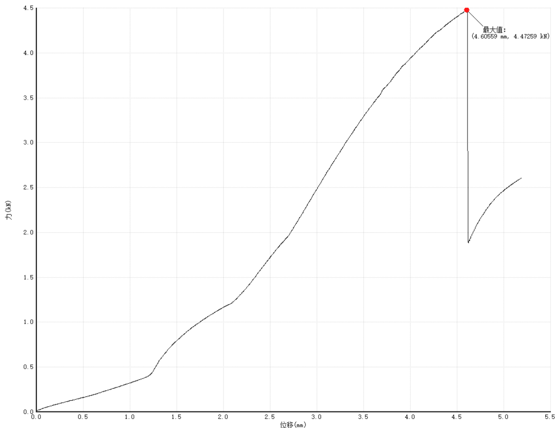
Force-displacement curve
