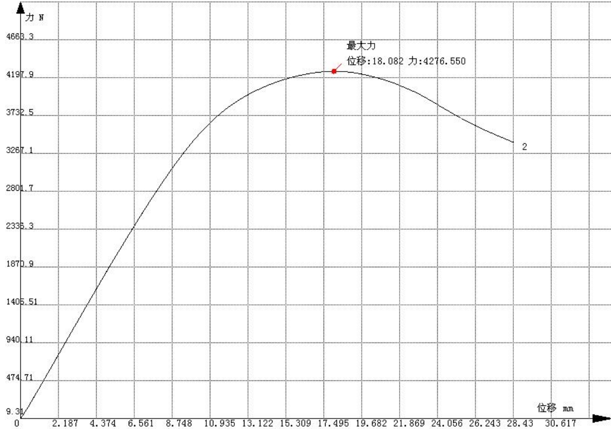
Force-displacement curve
