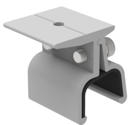
• WQ-AC-02 Laysaght Klip-lok 700 Clamp
