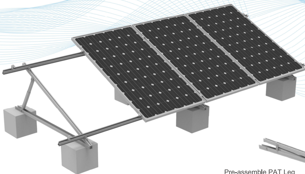
Pre-assemble PAT Leg
